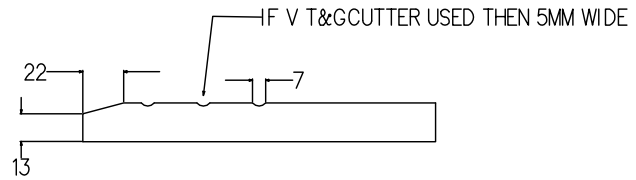
BEVELLED PROFILE WITH TRIPLE COVE
