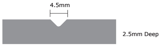
'V' Cutter
